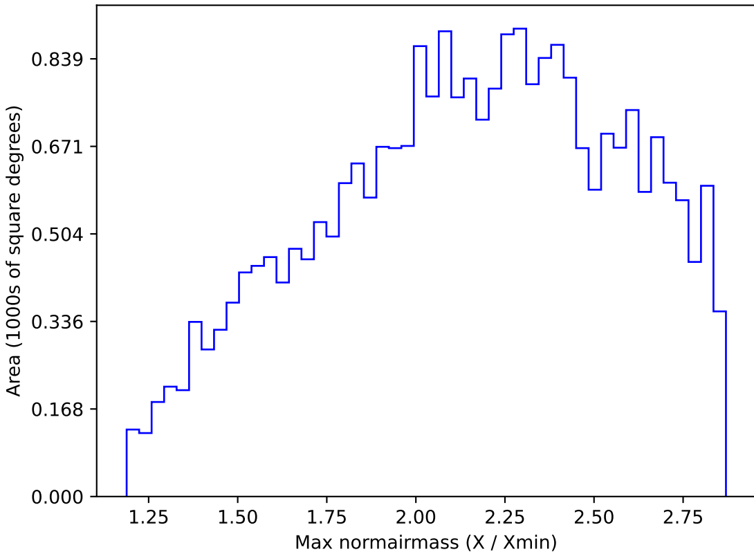
too_5_1v3.4_10yrs All sky z band: Max normairmass
