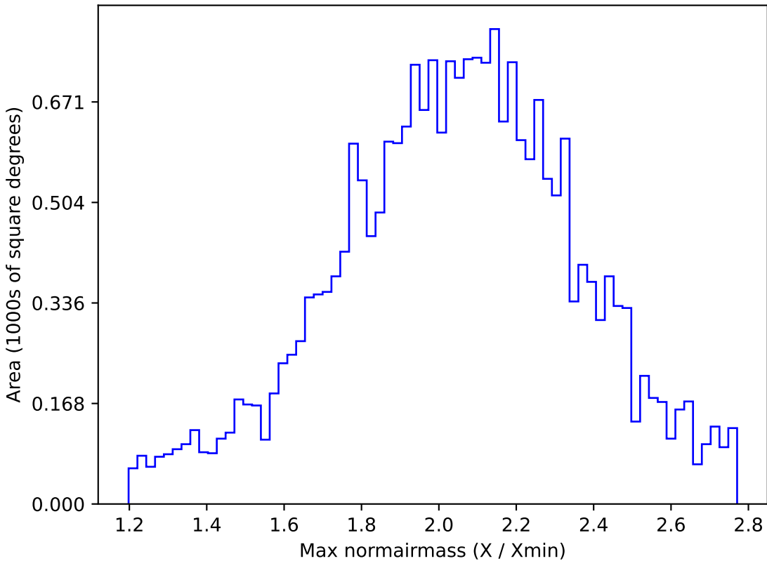
too_5_1v3.4_10yrs All sky y band: Max normairmass
