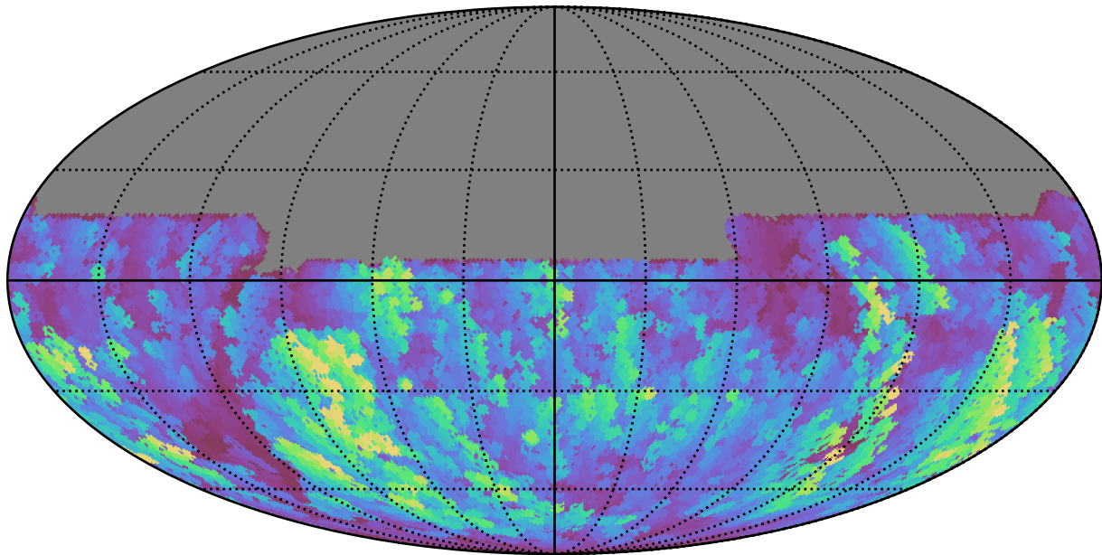
too_5_1v3.4_10yrs All sky u band: Max normairmass
