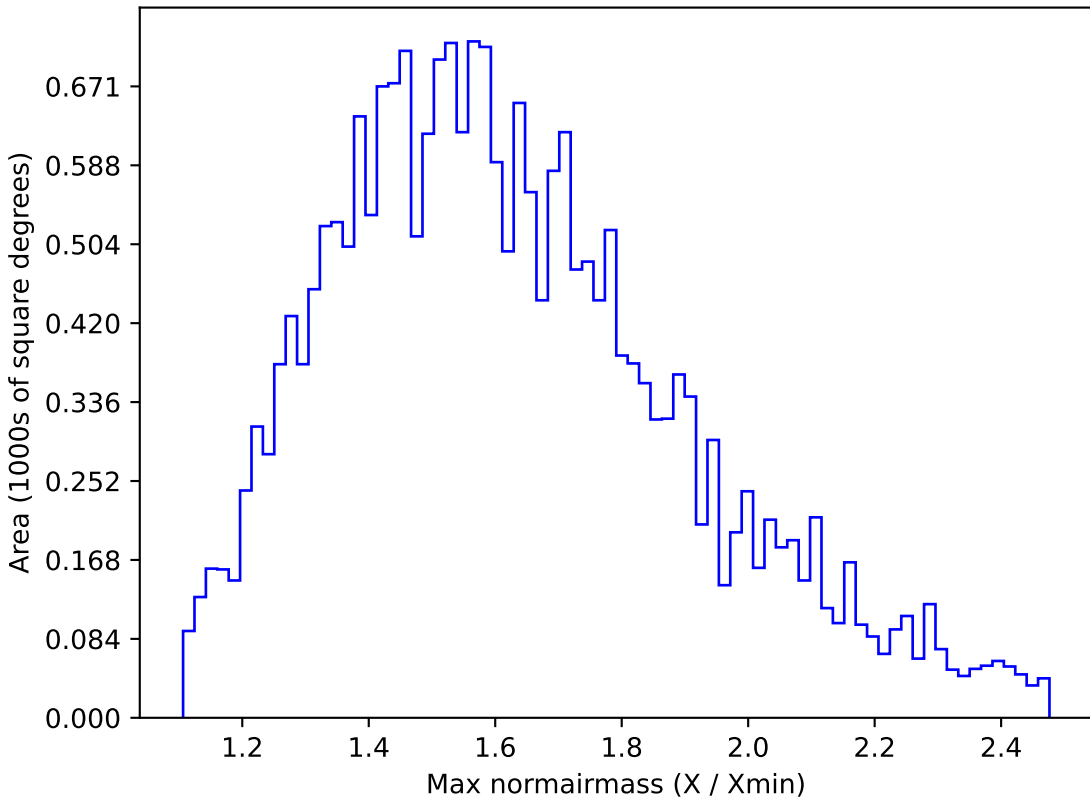
too_5_1v3.4_10yrs All sky u band: Max normairmass
