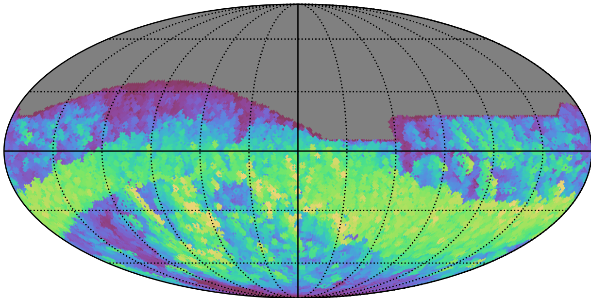
too_5_1v3.4_10yrs All sky r band: Max normairmass
