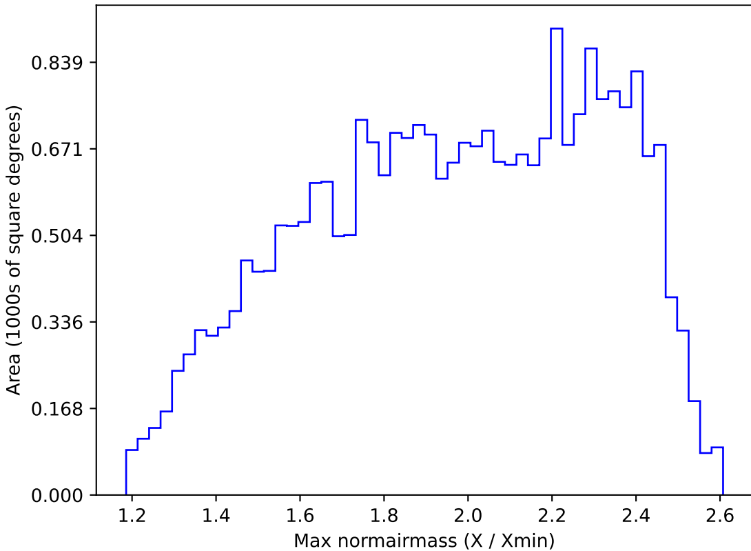
too_5_1v3.4_10yrs All sky r band: Max normairmass
