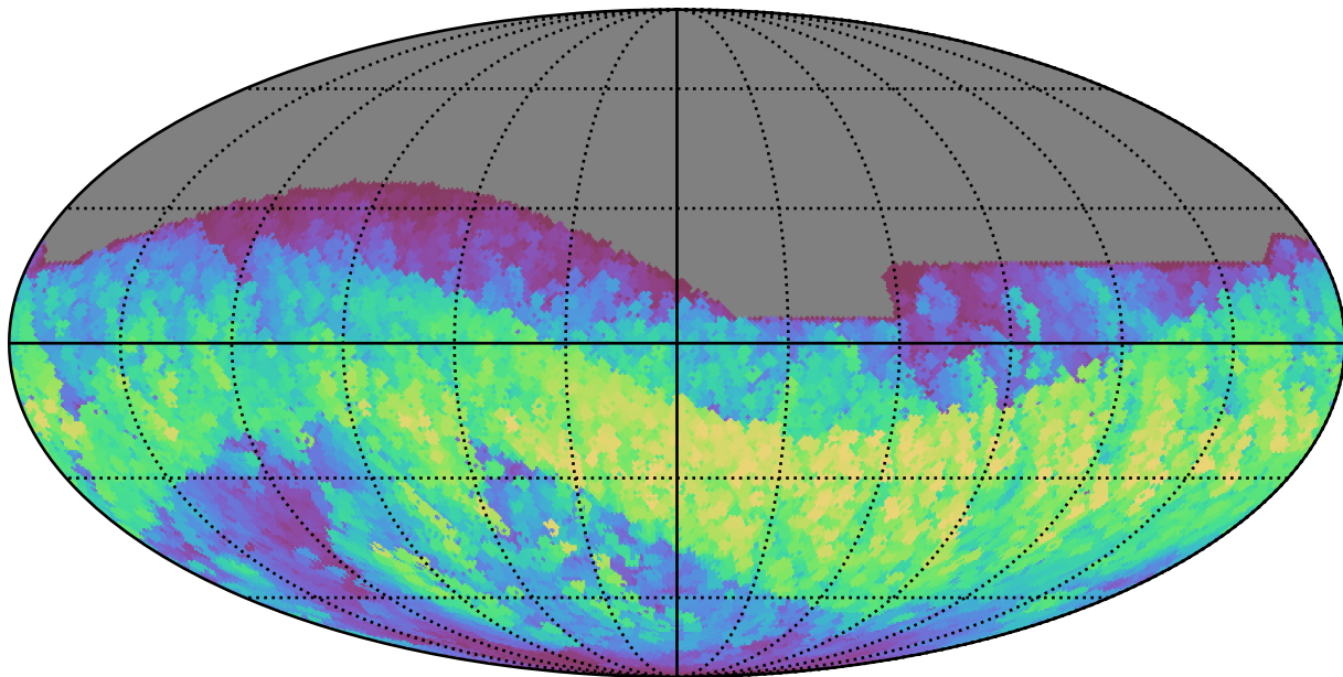
too_5_1v3.4_10yrs All sky i band: Max normairmass
