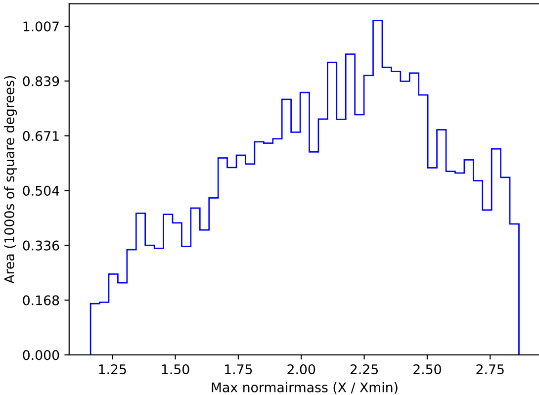
too_5_1v3.4_10yrs All sky i band: Max normairmass
