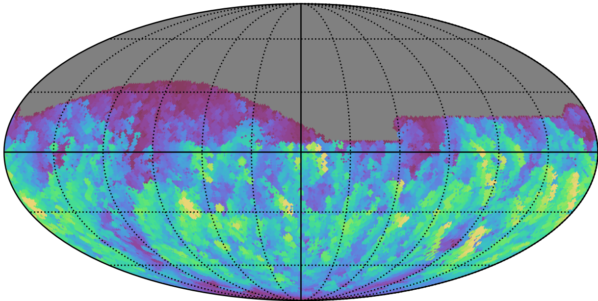
too_5_1v3.4_10yrs All sky g band: Max normairmass
