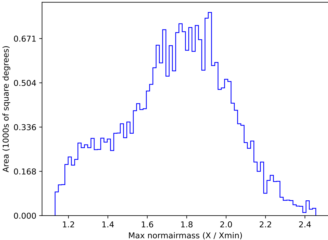
too_5_1v3.4_10yrs All sky g band: Max normairmass
