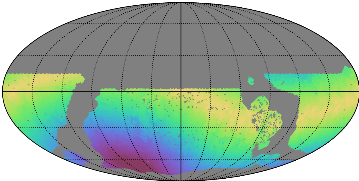
too_5_1v3.4_10yrs WFD z band: Max moonDistance
