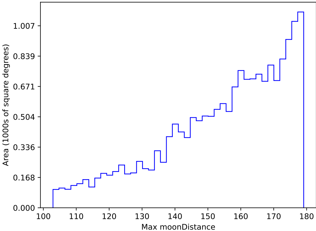
too_5_1v3.4_10yrs WFD z band: Max moonDistance
