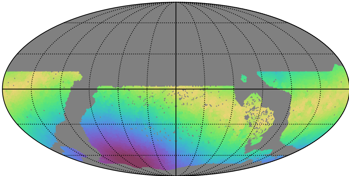
too_5_1v3.4_10yrs WFD g band: Max moonDistance
