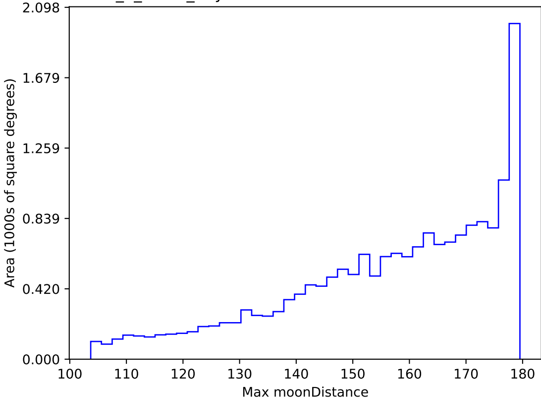
too_5_1v3.4_10yrs WFD all bands: Max moonDistance
