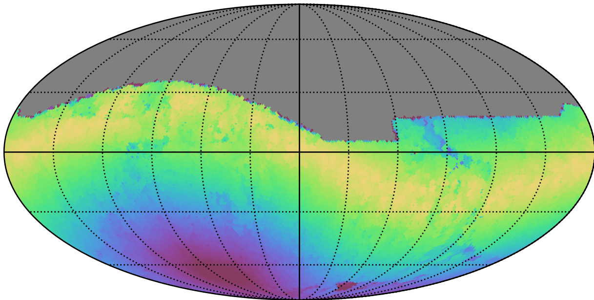
too_5_1v3.4_10yrs All sky z band: Max moonDistance
