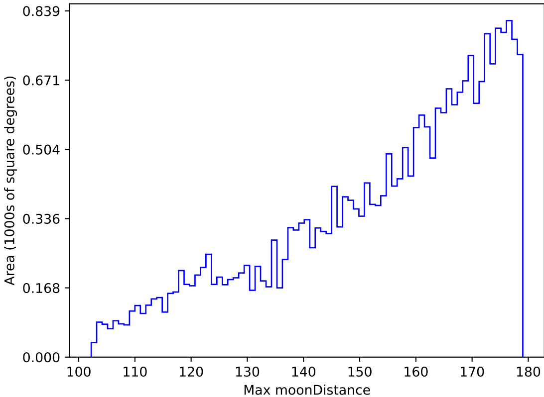
too_5_1v3.4_10yrs All sky z band: Max moonDistance
