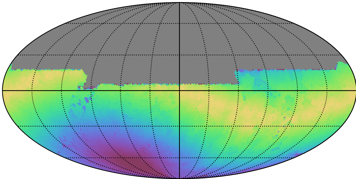
too_5_1v3.4_10yrs All sky u band: Max moonDistance
