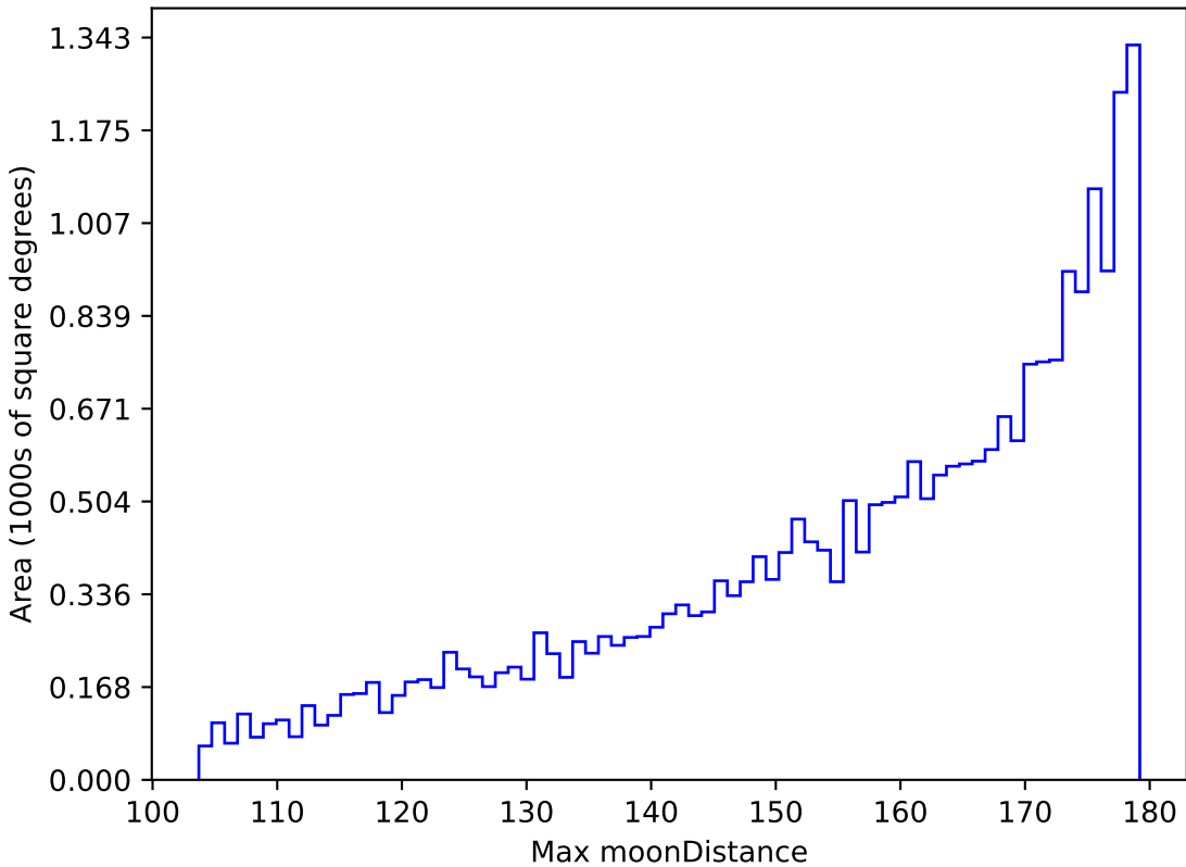
too_5_1v3.4_10yrs All sky r band: Max moonDistance
