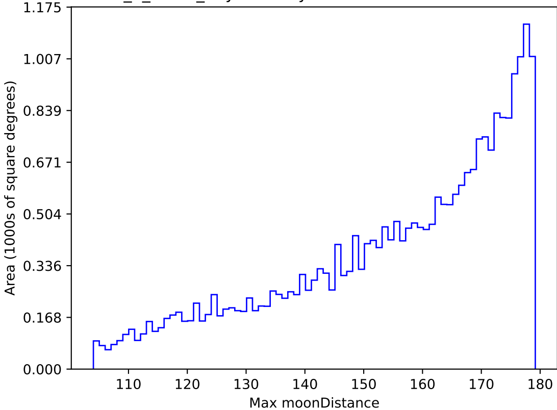
too_5_1v3.4_10yrs All sky i band: Max moonDistance
