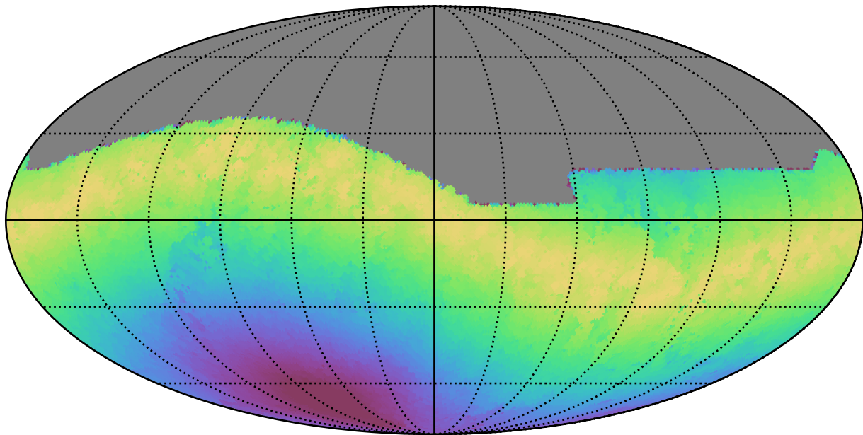
too_5_1v3.4_10yrs All sky g band: Max moonDistance
