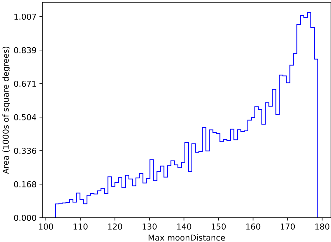
too_5_1v3.4_10yrs All sky g band: Max moonDistance
