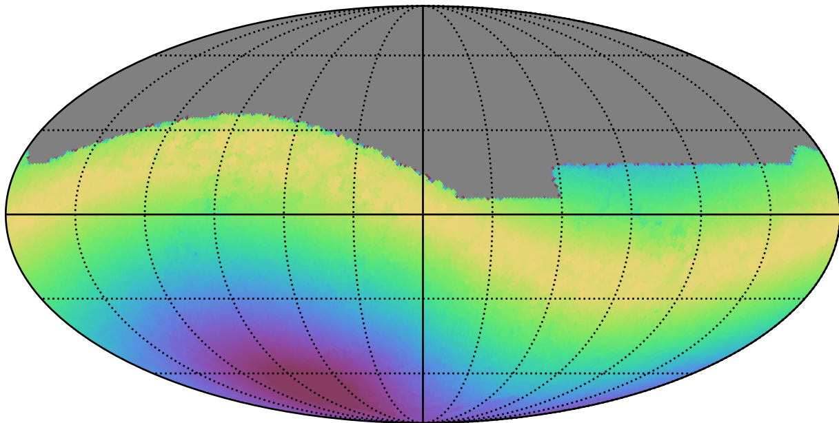
too_5_1v3.4_10yrs All sky all bands: Max moonDistance
