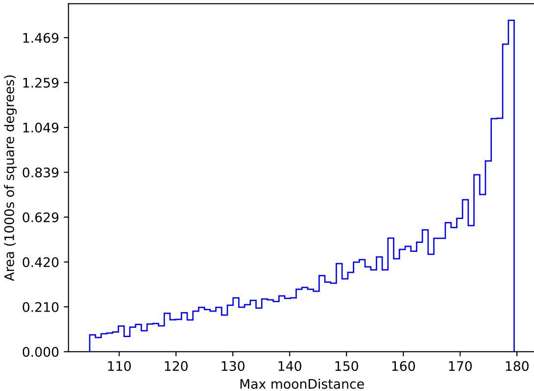
too_5_1v3.4_10yrs All sky all bands: Max moonDistance
