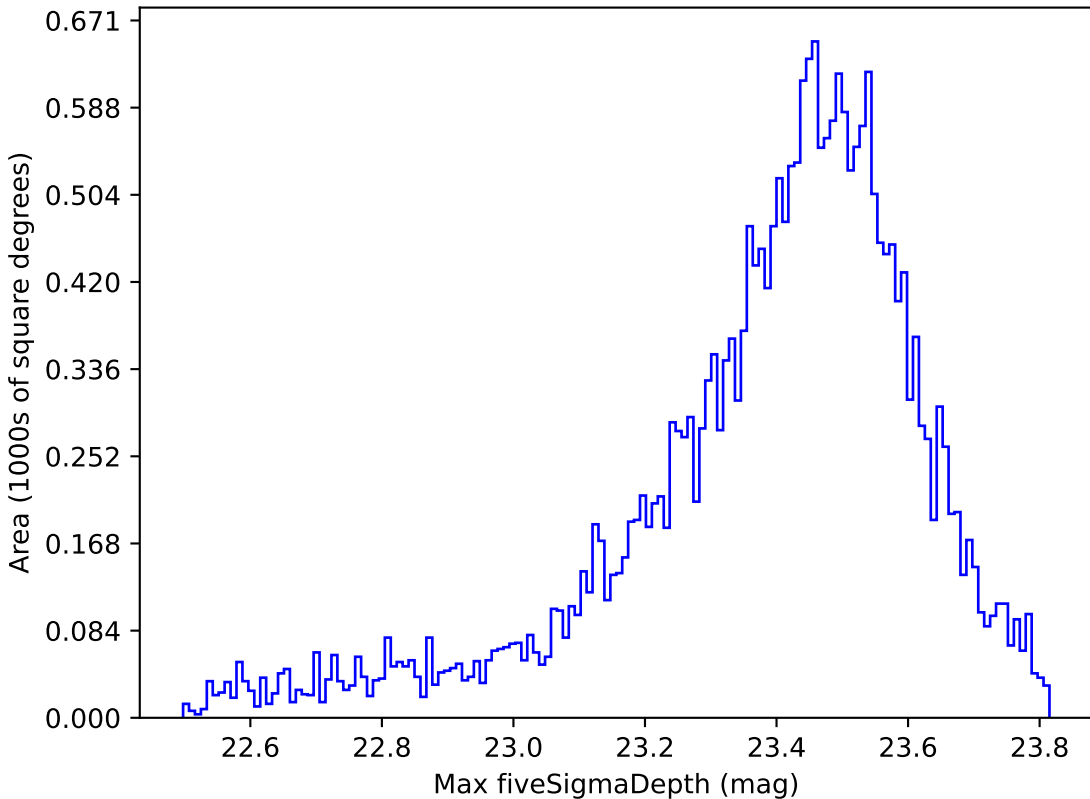
too_5_1v3.4_10yrs Yr 1 z band: Max fiveSigmaDepth
