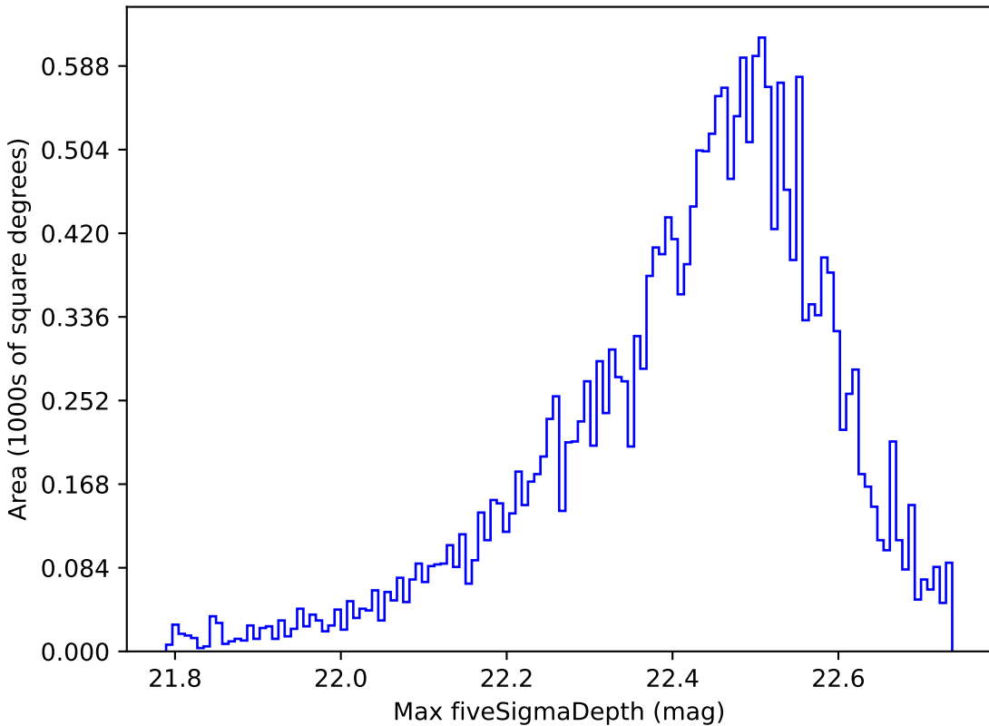
too_5_1v3.4_10yrs Yr 1 y band: Max fiveSigmaDepth
