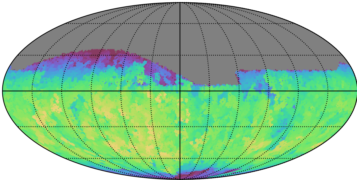
too_5_1v3.4_10yrs Yr 1 r band: Max fiveSigmaDepth
