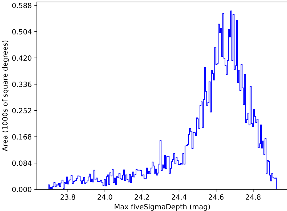
too_5_1v3.4_10yrs Yr 1 r band: Max fiveSigmaDepth
