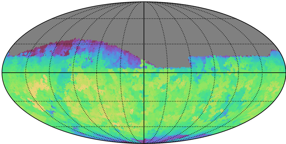
too_5_1v3.4_10yrs Yr 1 i band: Max fiveSigmaDepth
