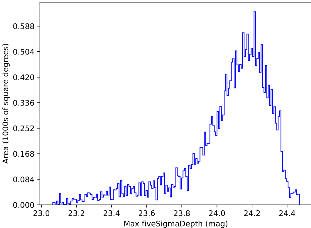
too_5_1v3.4_10yrs Yr 1 i band: Max fiveSigmaDepth
