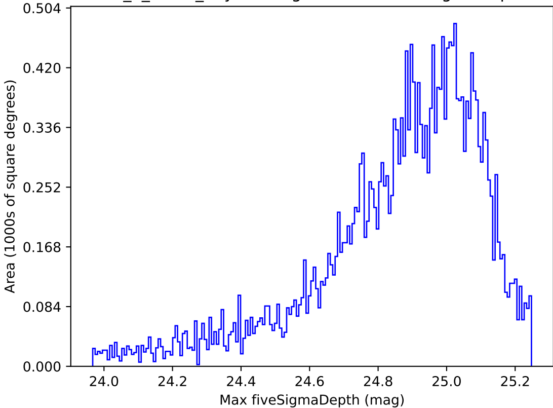
too_5_1v3.4_10yrs Yr 1 g band: Max fiveSigmaDepth
