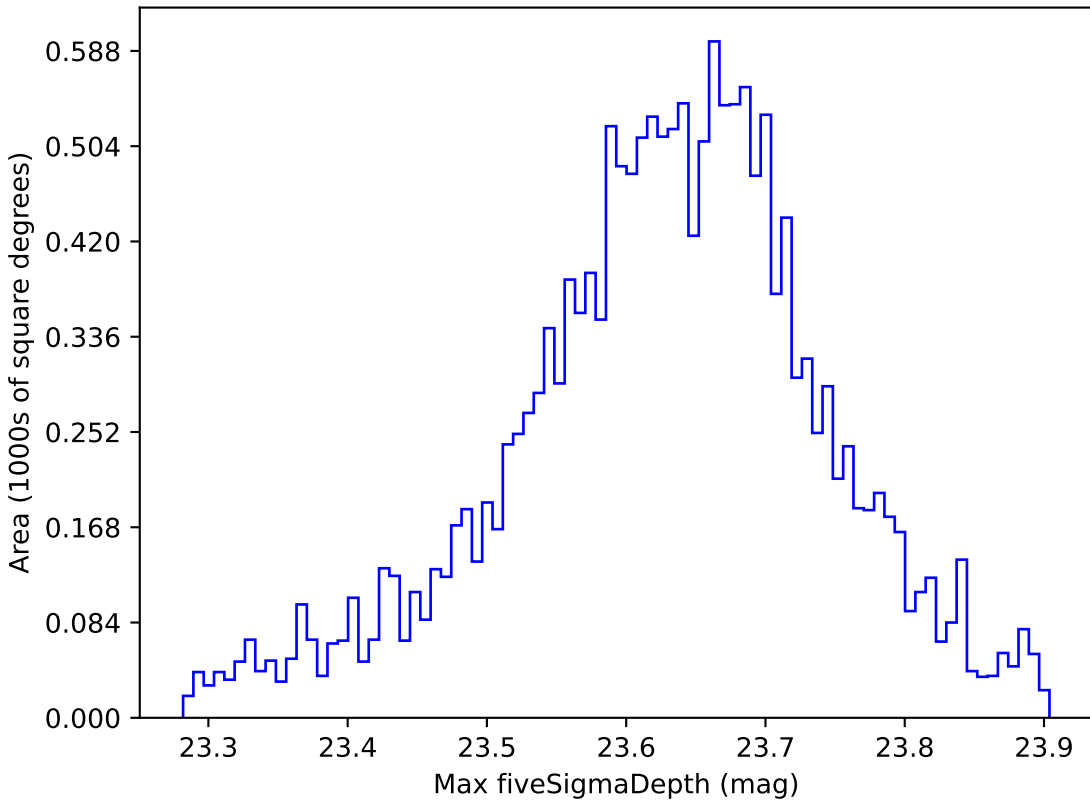
too_5_1v3.4_10yrs WFD z band: Max fiveSigmaDepth
