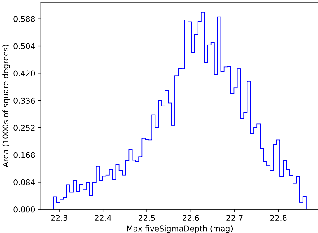
too_5_1v3.4_10yrs WFD y band: Max fiveSigmaDepth
