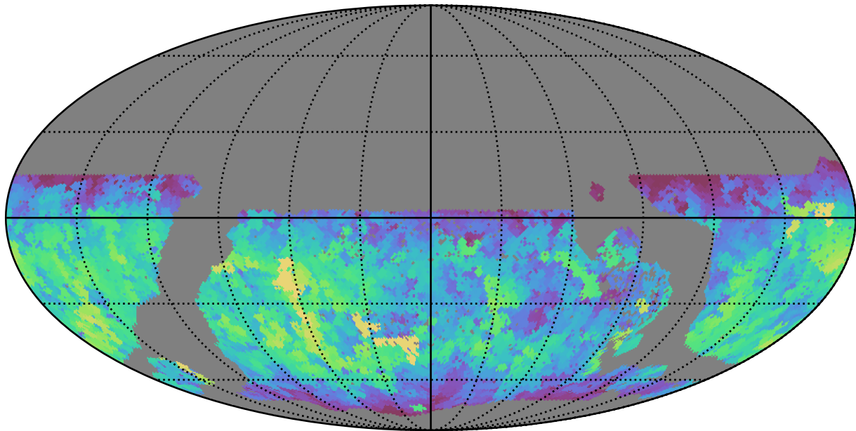
too_5_1v3.4_10yrs WFD u band: Max fiveSigmaDepth
