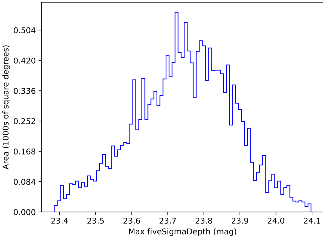
too_5_1v3.4_10yrs WFD u band: Max fiveSigmaDepth
