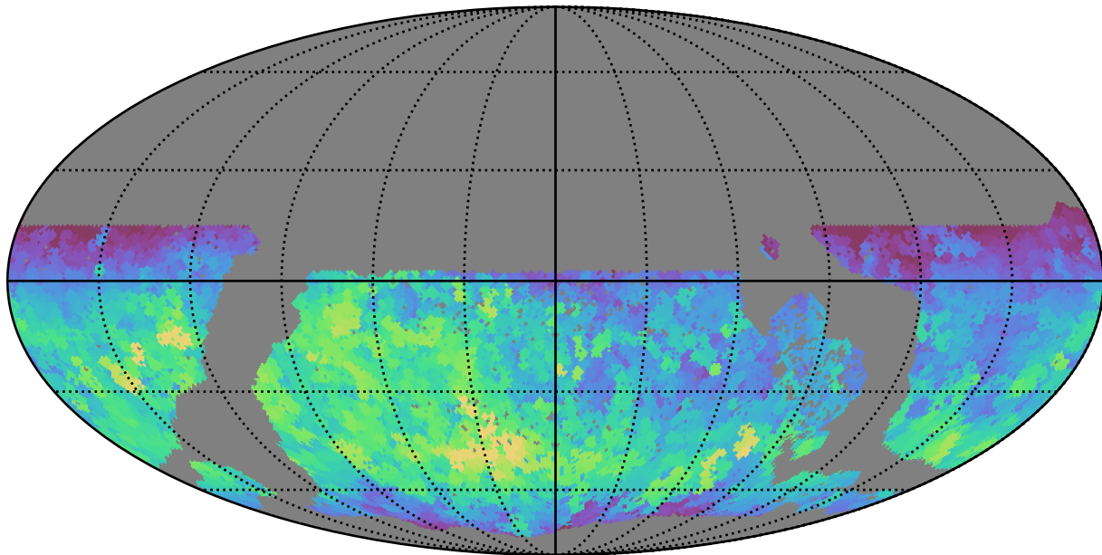
too_5_1v3.4_10yrs WFD r band: Max fiveSigmaDepth
