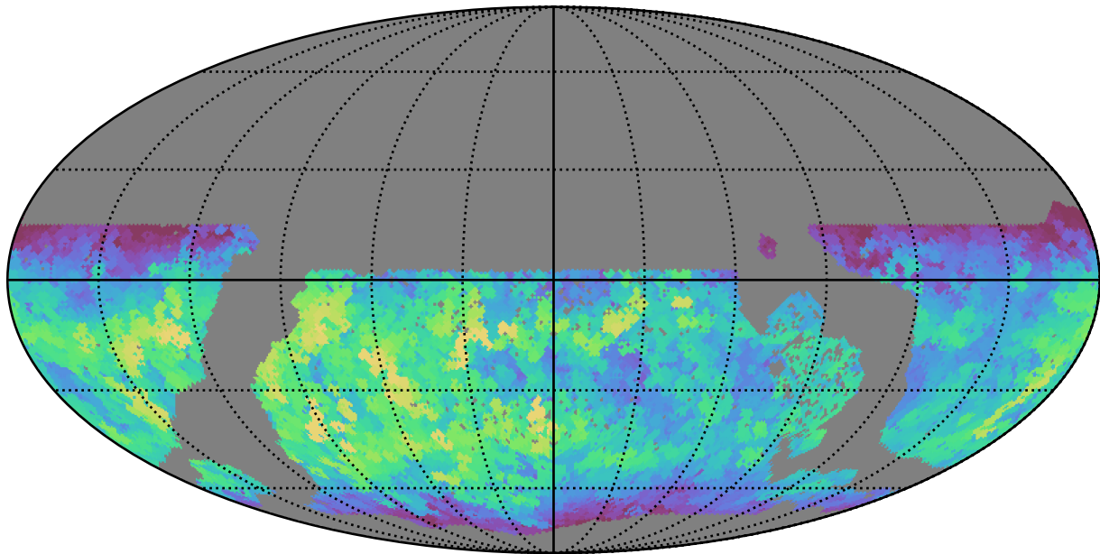
too_5_1v3.4_10yrs WFD i band: Max fiveSigmaDepth
