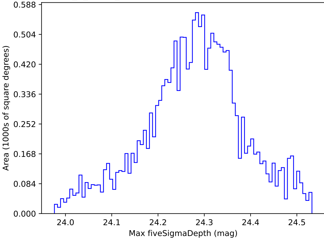
too_5_1v3.4_10yrs WFD i band: Max fiveSigmaDepth
