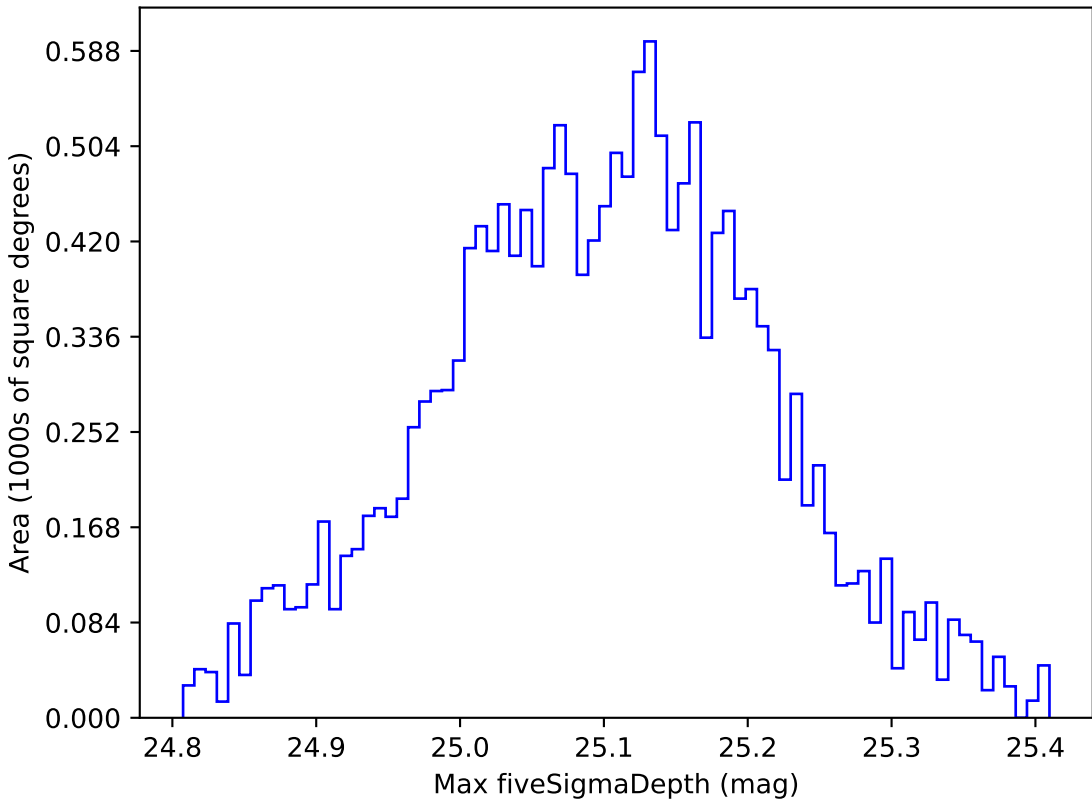
too_5_1v3.4_10yrs WFD g band: Max fiveSigmaDepth
