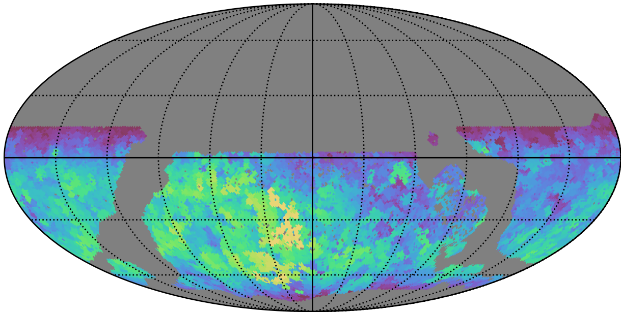
too_5_1v3.4_10yrs WFD all bands: Max fiveSigmaDepth
