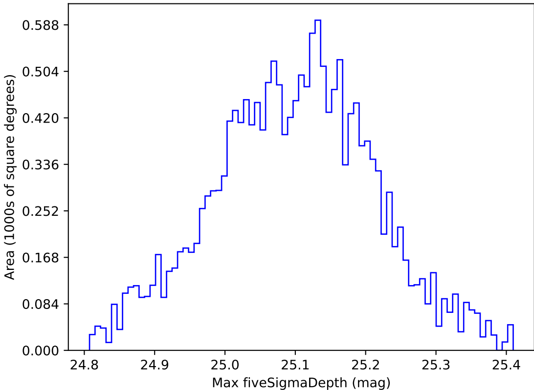
too_5_1v3.4_10yrs WFD all bands: Max fiveSigmaDepth
