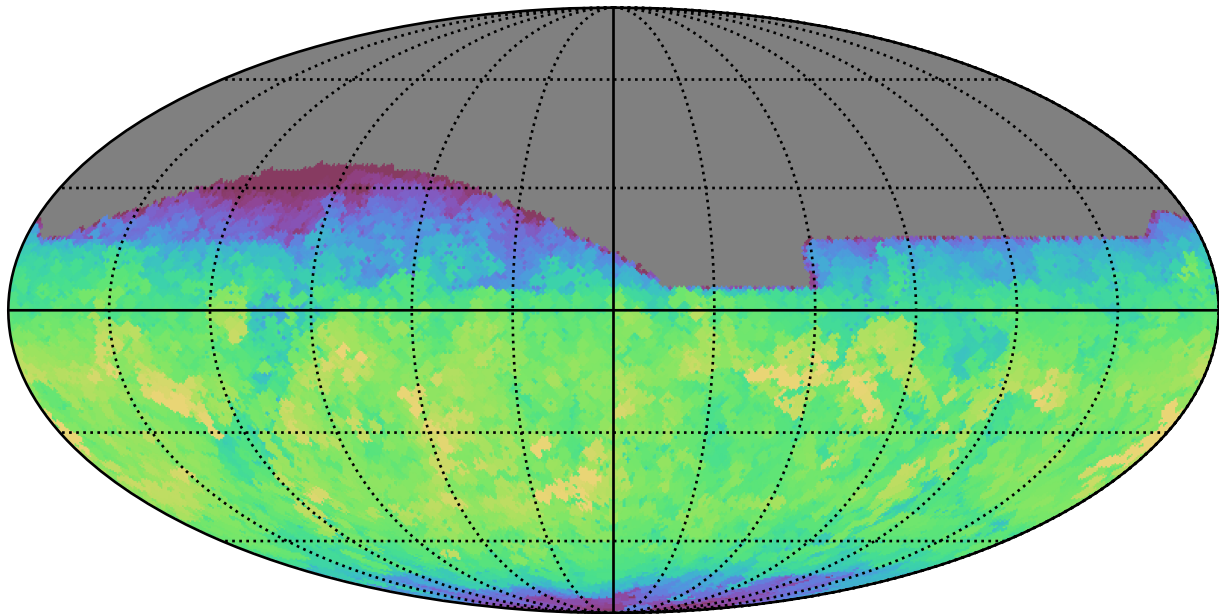
too_5_1v3.4_10yrs All sky z band: Max fiveSigmaDepth
