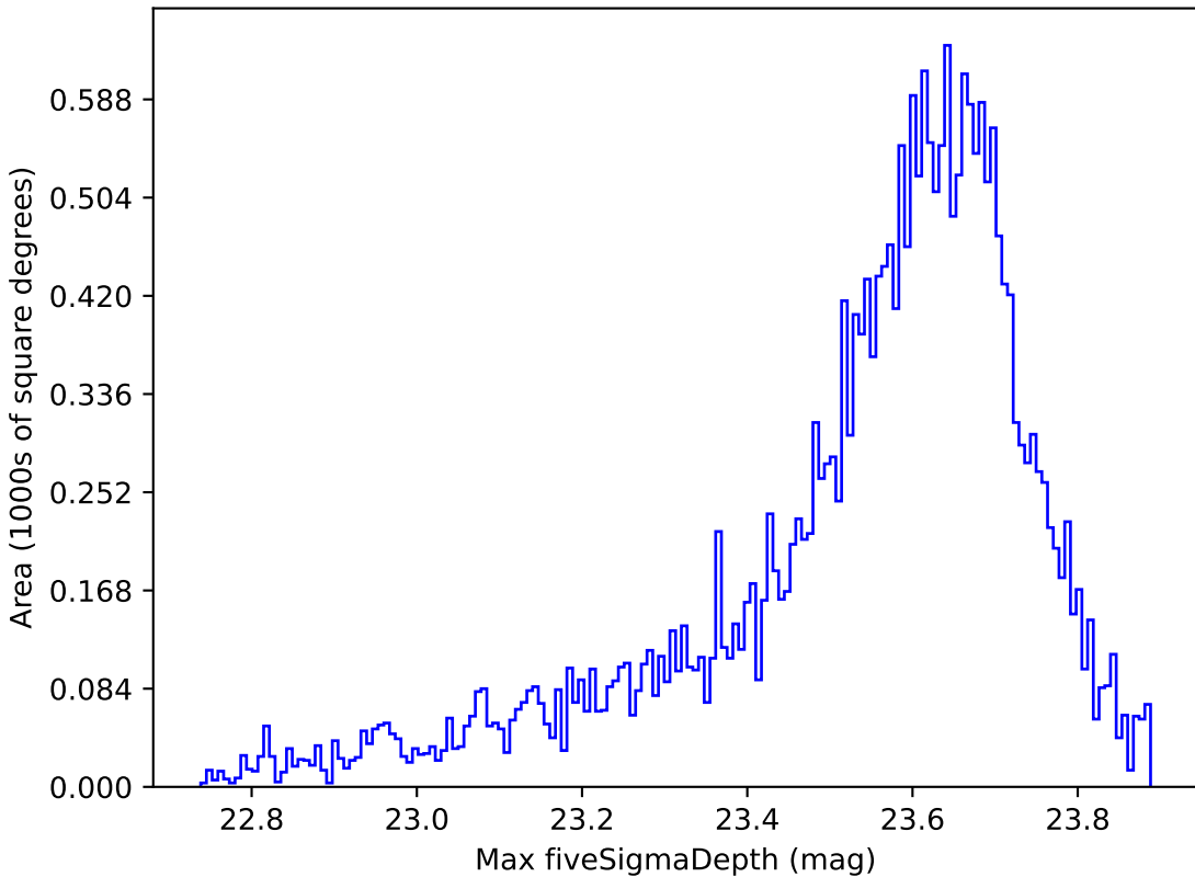
too_5_1v3.4_10yrs All sky z band: Max fiveSigmaDepth
