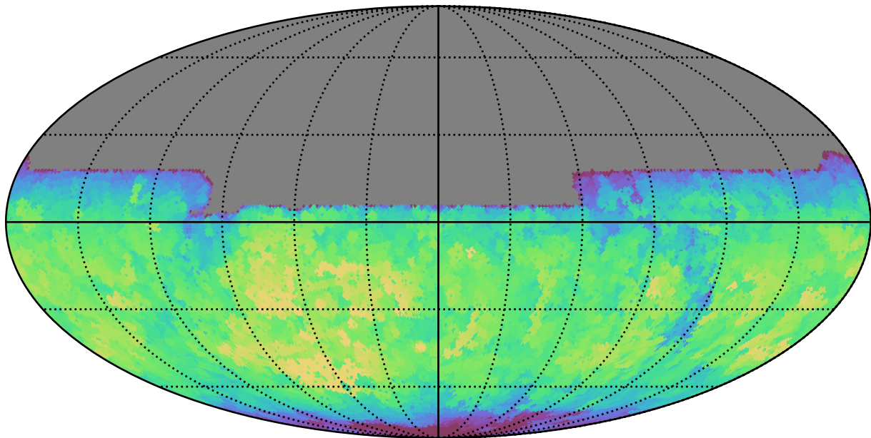
too_5_1v3.4_10yrs All sky y band: Max fiveSigmaDepth
