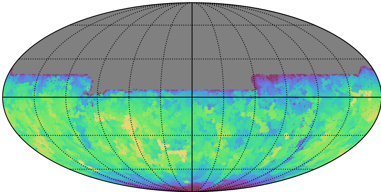
too_5_1v3.4_10yrs All sky u band: Max fiveSigmaDepth
