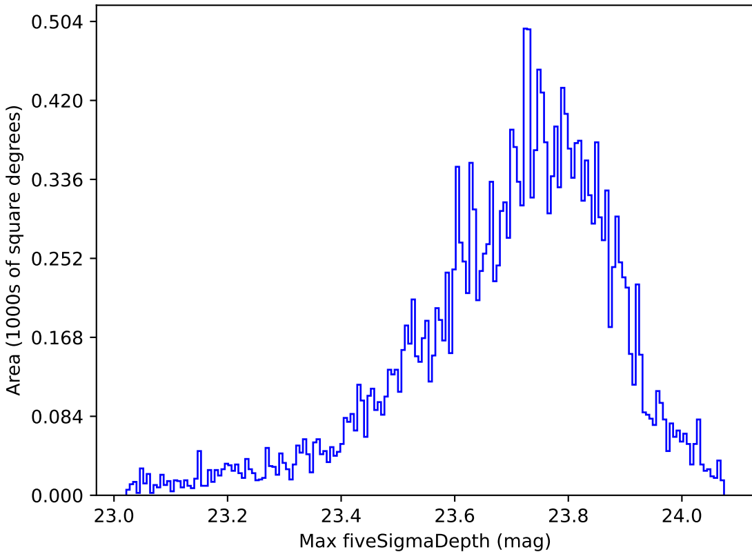
too_5_1v3.4_10yrs All sky u band: Max fiveSigmaDepth
