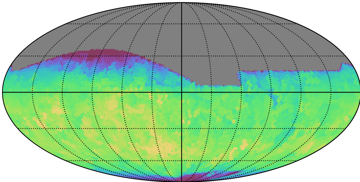
too_5_1v3.4_10yrs All sky r band: Max fiveSigmaDepth
