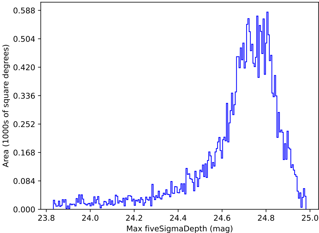
too_5_1v3.4_10yrs All sky r band: Max fiveSigmaDepth
