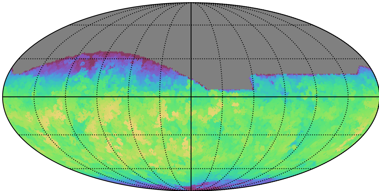
too_5_1v3.4_10yrs All sky i band: Max fiveSigmaDepth
