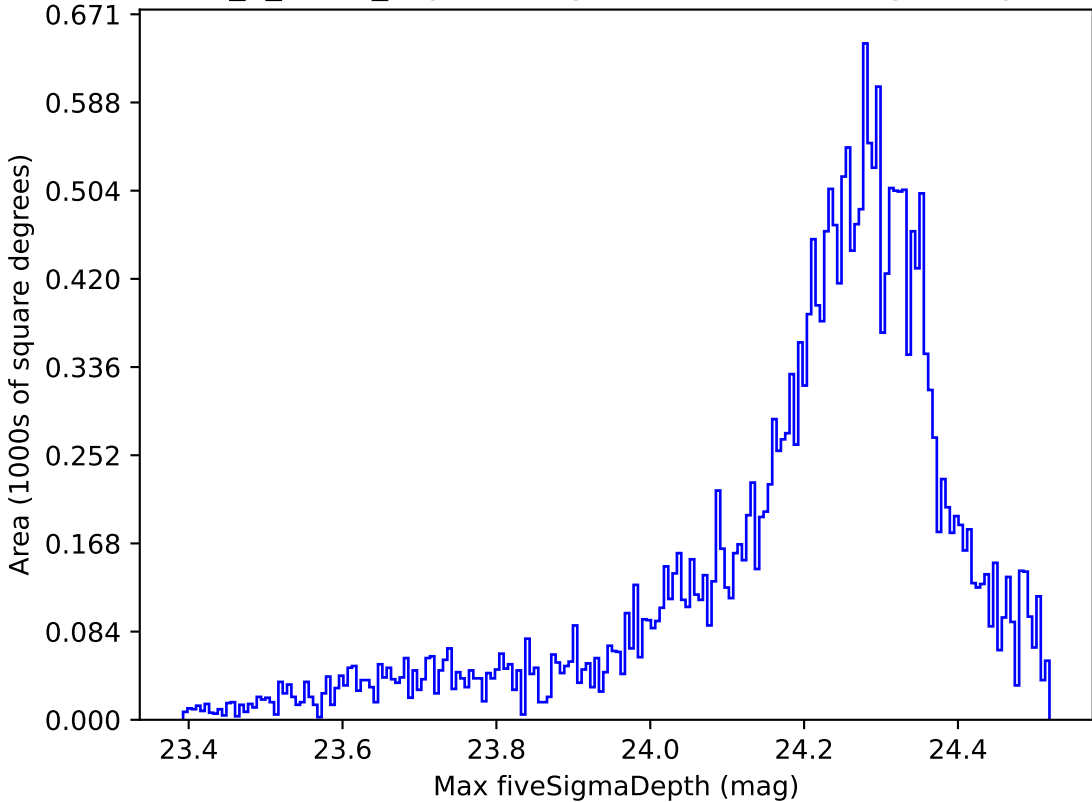
too_5_1v3.4_10yrs All sky i band: Max fiveSigmaDepth
