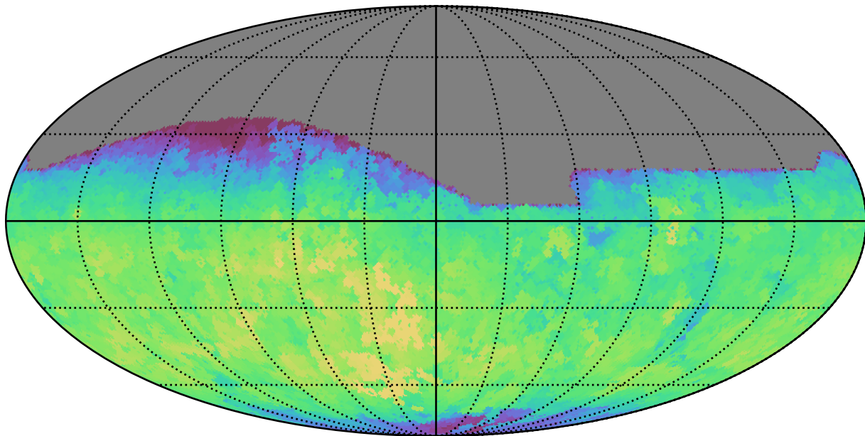
too_5_1v3.4_10yrs All sky g band: Max fiveSigmaDepth
